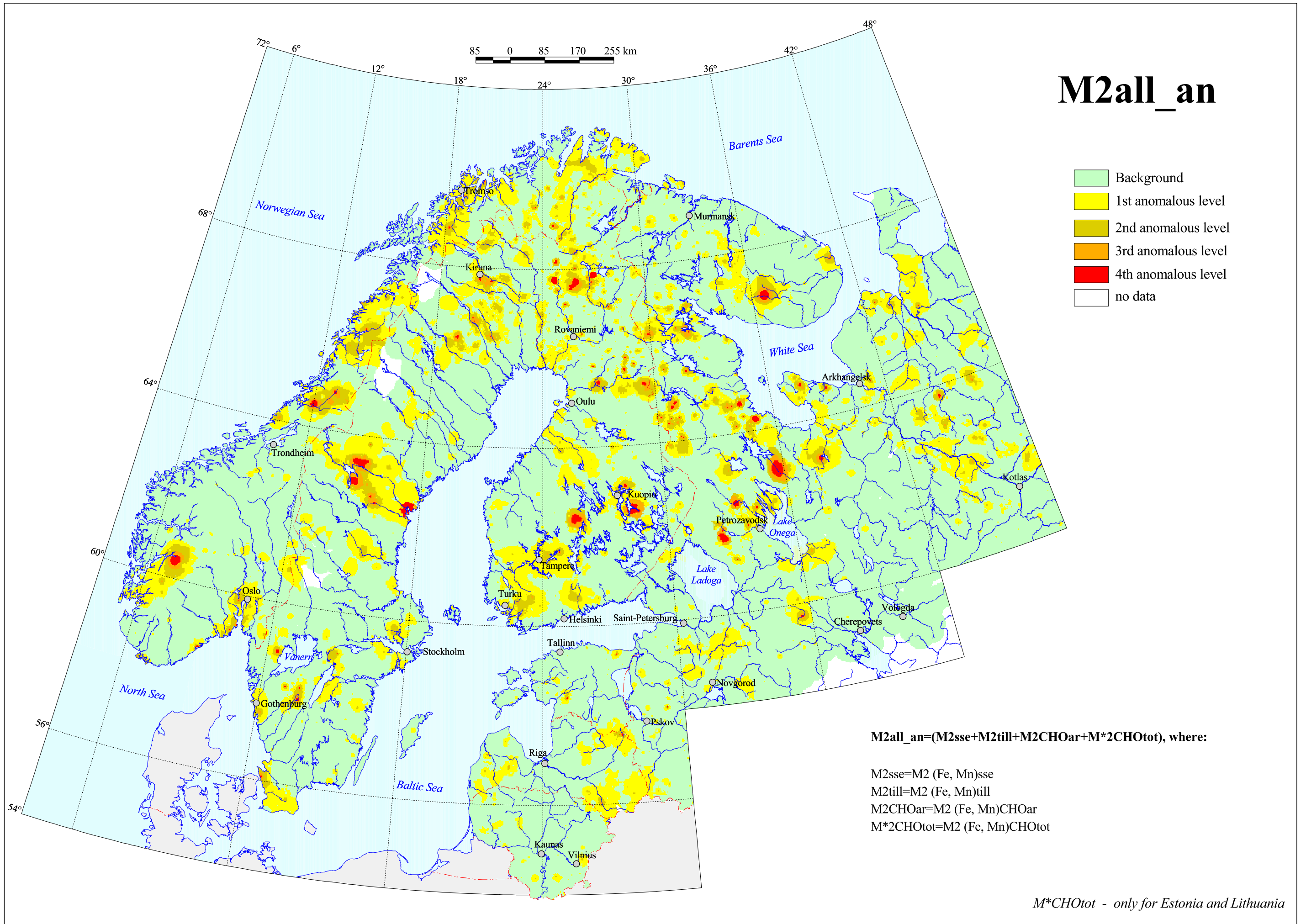
Integrated Anomalous Geochemical Fields, M2all_an
